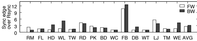
Fig. 6: Traversed edge of Sync over Rsync bottom-up.
