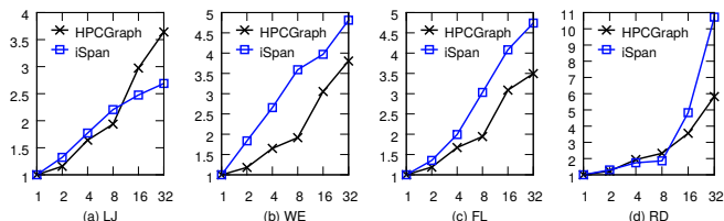
Fig. 15: The distributed scalability comparison (x-axis shows the number of nodes, y-axis shows the speedup).
